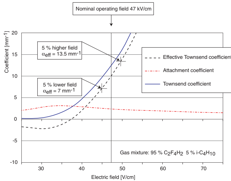
Fig. 2. Townsend coefficient, attachment coefficient and effective Townsend coefficient plotted versus electric field for a gas mixture of 5% isobutane and 95% C_2F_4H_2 . The 2 mm gap RPC is normally operated with an effective Townsend coefficient of 10, corresponding to an electric field of 47 kV/cm. The value of effective Townsend coefficient for a change of electric field of \pm 5\% are marked on this figure
