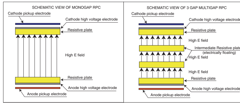
Fig. 1. Schematic representation of monogap and multigap RPC
