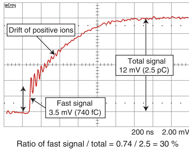
Fig. 4. Induced charge caused by charged particle passing through a 10 gap RPC with gap size of 250\ \mu\text{m} . The readout electrodes were connected to the high impedance input of a digital oscilloscope so that the voltage represented the total collected charge at that point. By knowing the capacitance ( 212\ \text{pF} in this case), the correspondence between voltage and charge is given
